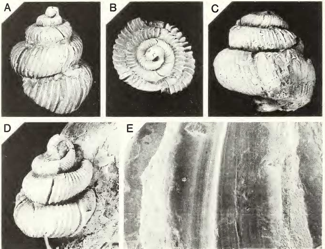
TEXT-FIG. 1. Eubostrychoceras muramotoi Matsumoto. A, WEA 003T-1, from Obirashibe River (near mouth of Okufutamata-zawa tributary), Obira area; Coniacian; lateral view, \times 1.5 . B, apical view of the same specimen, \times 1.5 . C, WEA 004T, from the same locality; lateral view of sinistral specimen, \times 1 . D, GK.H5589 from Pombetsu, Go-no-sawa, Ikushumbetsu area; Coniacian; upper view of holotype, \times 2 . E, WEA 003T-2, from the same locality as specimen in A; SEM photograph indicating conformable relation between ribs and growth lines, \times 25 .
